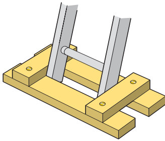
Figure 7 Tying at the base
